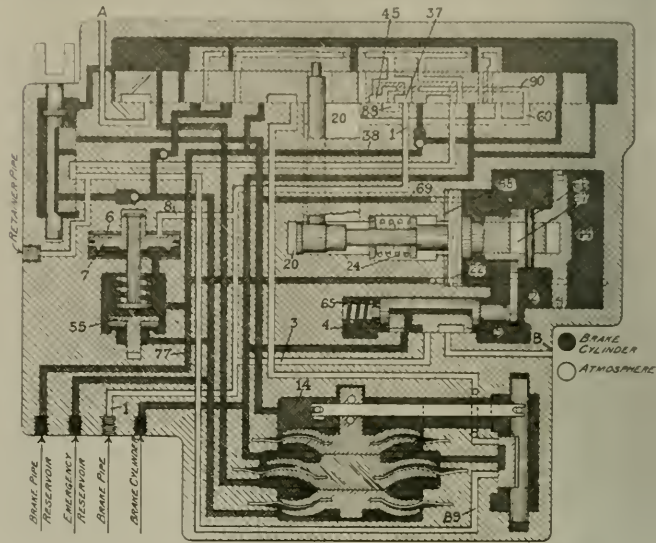
FIG. 7. EMERGENCY LAP POSITION - TRIPLE VALVE IN QUICK RELEASE
